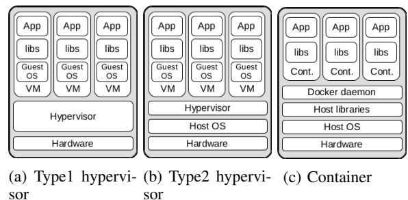
Fig. 1: Application runtime models
